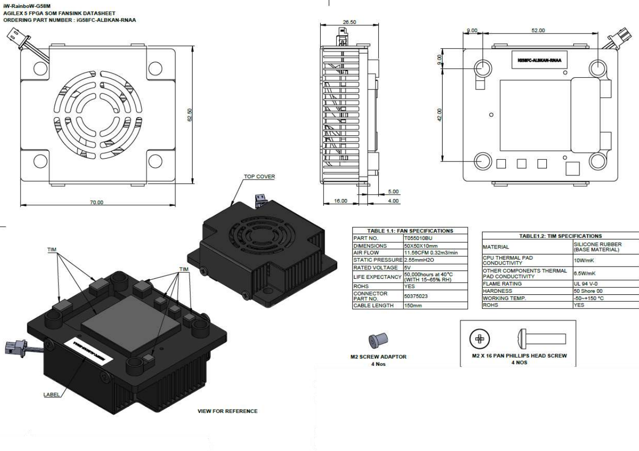
Figure 9: FANSINK
