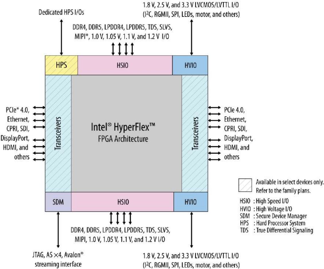
Figure 2: Altera Agilinx 5 E-series SoC FPGA (B32A) SOC Block Diagram
