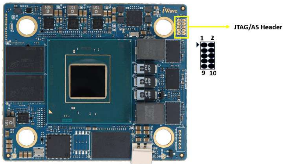
Figure 4: JTAG/Active Serial Header
