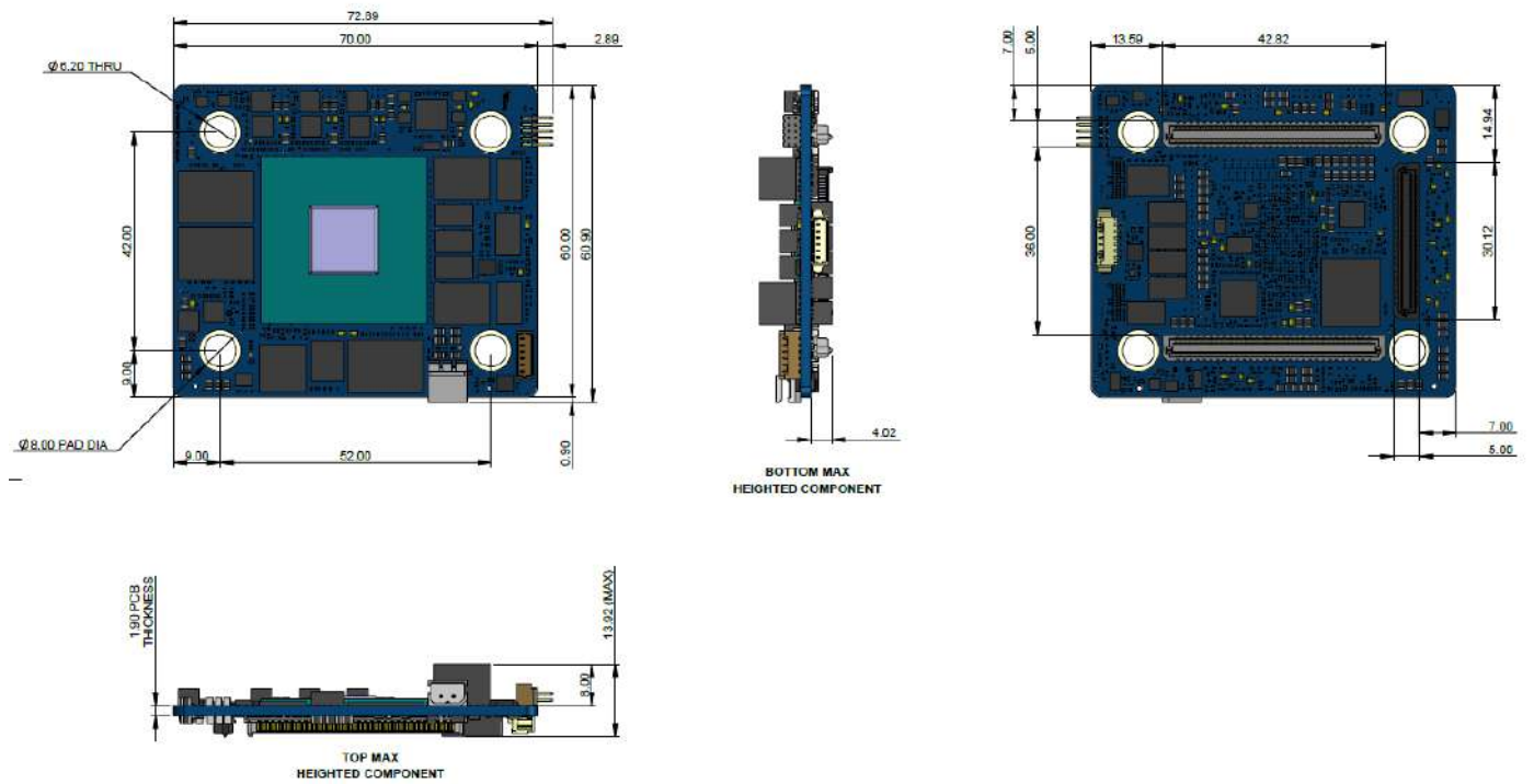
Figure 10: Mechanical dimension of Altera Agilex 5 SoC FPGA SOM
