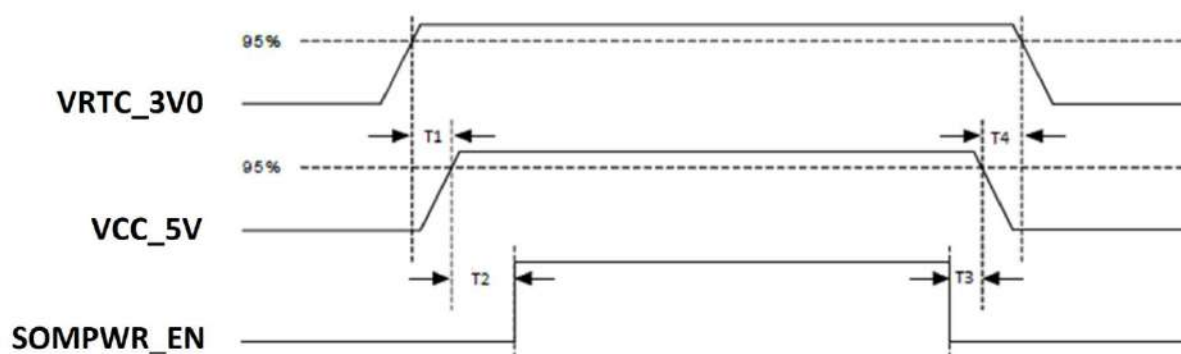
Figure 8: Power Input Sequencing
